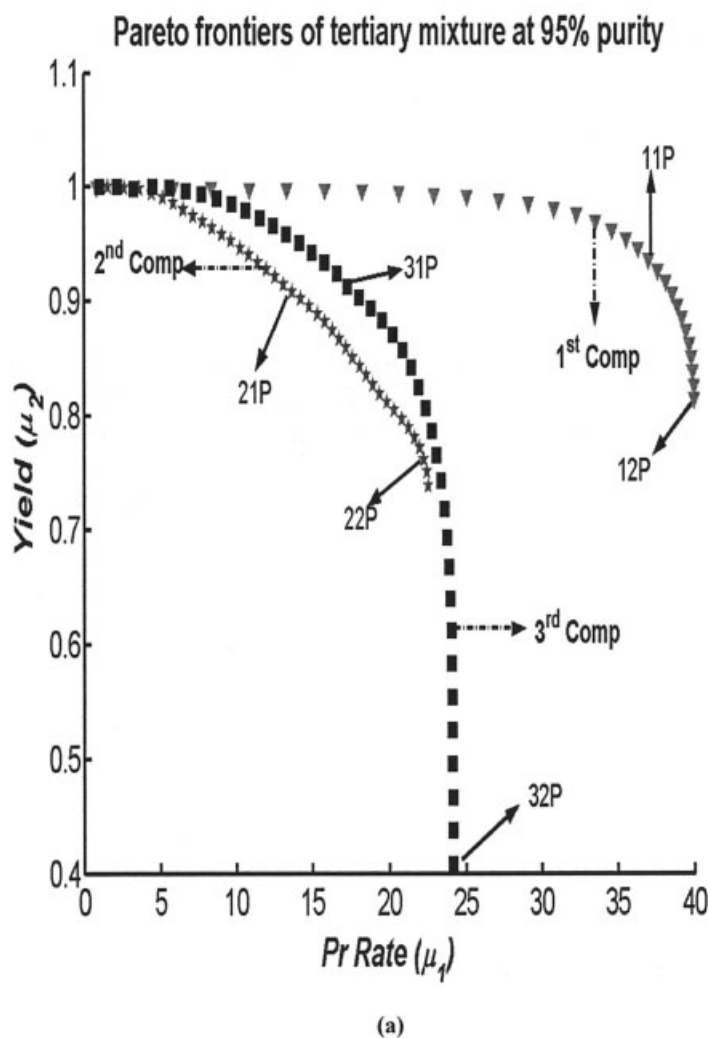
Figure 7. Pareto frontiers and outlet concentration profiles for a tertiary mixture ( \alpha -chymotrypsinogen A, ribonuclease A, and artificial component) on a 90 \mu\text{m} FF Sepharose stationary phase.
