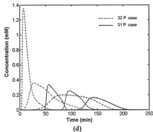
Figure 7. Pareto frontiers and outlet concentration profiles for a tertiary mixture ( \alpha -chymotrypsinogen A, ribonuclease A, and artificial component) on a 90 \mu\text{m} FF Sepharose stationary phase.
